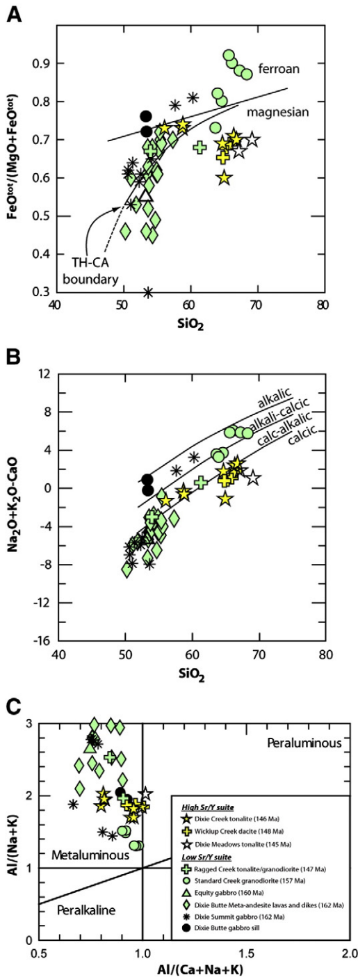
Fig. 7. Major element geochemical plots for plutonic and volcanic rocks in the Dixie Butte area. (A) FeO^{tot}/(FeO^{tot} + MgO) versus weight percent SiO_2 . (B) Plot of Na_2O + K_2O - CaO versus SiO_2 . (C) Alumina saturation indices indicating the metaluminous to peraluminous character of the plutonic rocks in the Dixie Butte area.
